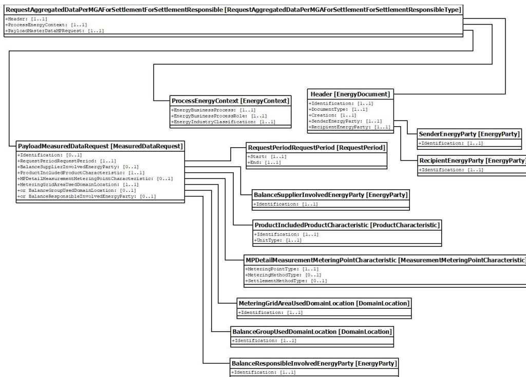
Slika 4: Dijagram klase za XML šemu RequestAggregatedDataPerMGAFForSettlementForSettlementResponsible
